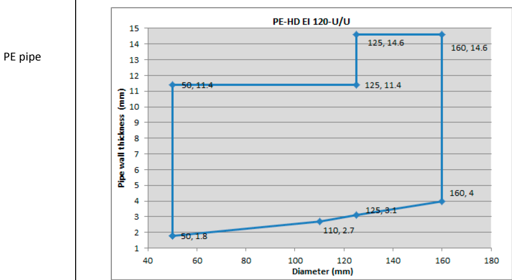
Illustrated classified pipe dimensions
